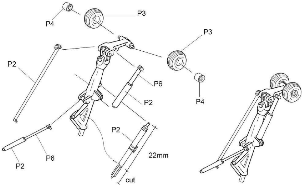
Train Dr / Right landing gear
